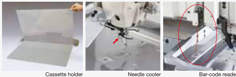
Cassette holder
