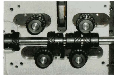
Adjustable gears allow use of any needle combination
