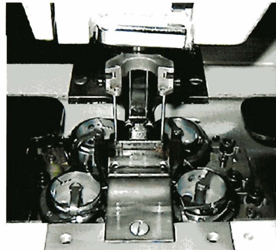
Four Horizontal Hooks and Bobbins
