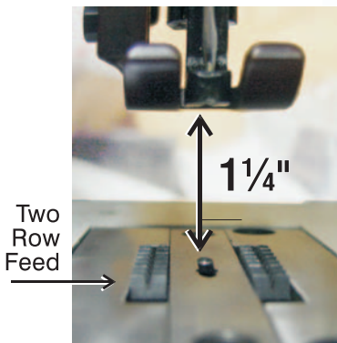
Detail of 733R-5 showing the two row feeder and the 1-1/4" extra high lift
